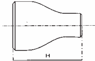
CONC. REDUCER
