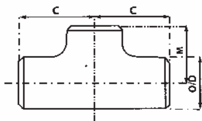
EQUAL TEE
