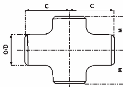
EQUAL CROSS
